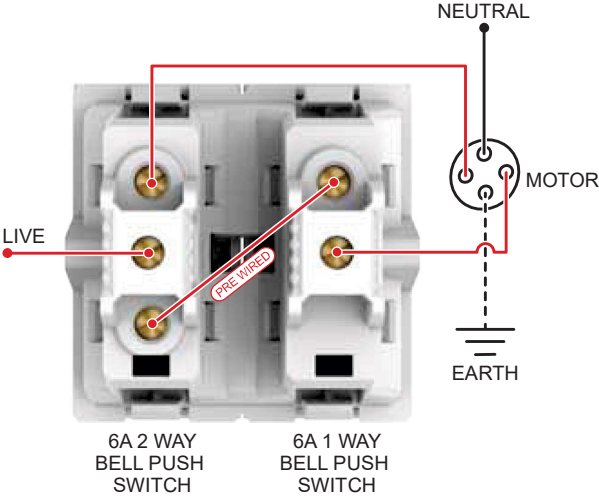
> Curtain Control Switch UNSCURTAINSW2M_WE
