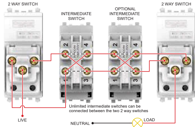
> 10AX Intermediate Switch IN8430/IM, IN8430/IM (BZ)
