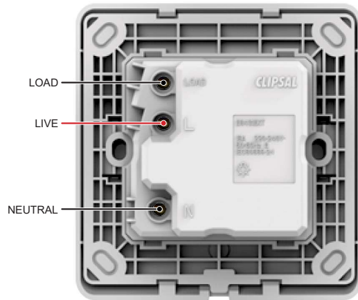
> 16A Electronic Keycard Switch CPXKEYCARDSW_WE, CPXKEYCARDSW_GY
