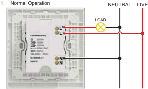
> PIR Motion Sensor* UNSPIR_WE
